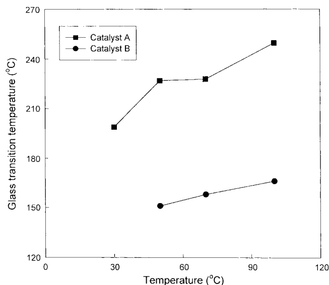
Fig. 3. Glass transition temperatures of ethylene-norbornene copolymers produced at different polymerization temperatures with a constant ethylene pressure (4.1 bar). Catalyst A = 2,2'-CH 2 (1,3-Me 2 Cp) 2 ZrCl 2 , Catalyst B = rac -Et(Ind) 2 ZrCl 2 .
