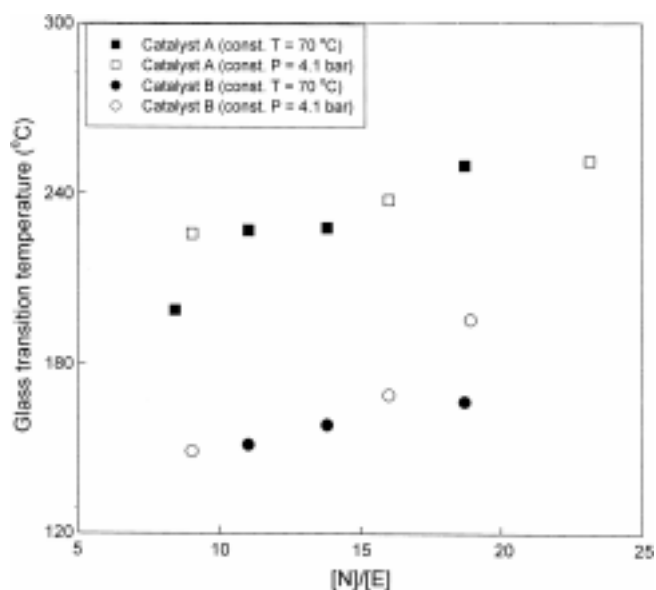
Fig. 5. Glass transition temperature of ethylene-norbornene copolymers produced as a function of norbornene/ethylene mole ratio in the reaction medium. Catalyst A = 2,2'-CH 2 (1,3-Me 2 Cp) 2 ZrCl 2 , Catalyst B = rac -Et(Ind) 2 ZrCl 2 .
