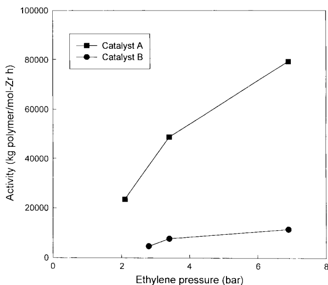
Fig. 2. Catalyst activities of ethylene-norbornene copolymers produced at different ethylene pressures with a constant temperature (70 °C). Catalyst A=2,2'-CH 2 (1,3-Me 2 Cp) 2 ZrCl 2 , Catalyst B= rac -Et(Ind) 2 ZrCl 2 .
