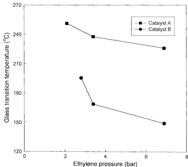
Fig. 4. Glass transition temperatures of ethylene-norbornene copolymers produced at different ethylene pressures with a constant temperature (70 °C). Catalyst A = 2,2'-CH 2 (1,3-Me 2 Cp) 2 ZrCl 2 , Catalyst B = rac -Et(Ind) 2 ZrCl 2 .
